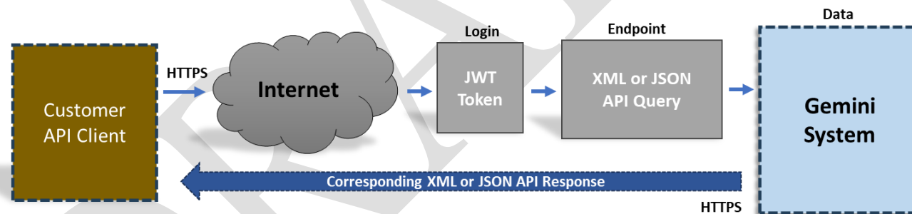
Figure 2.1: API Flow Overview
