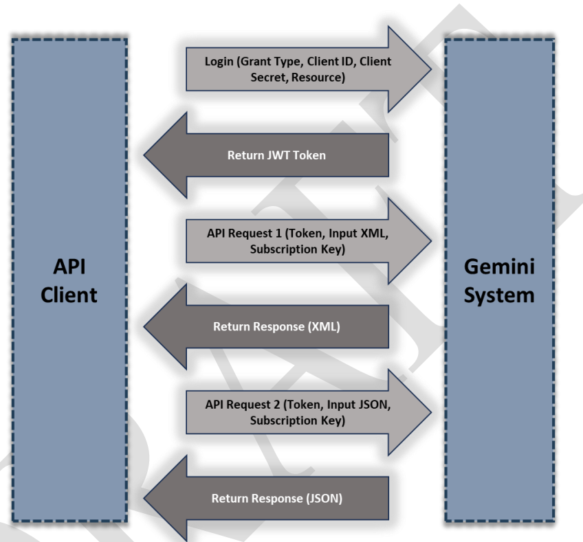
Figure 2.2: API Sequence Overview
